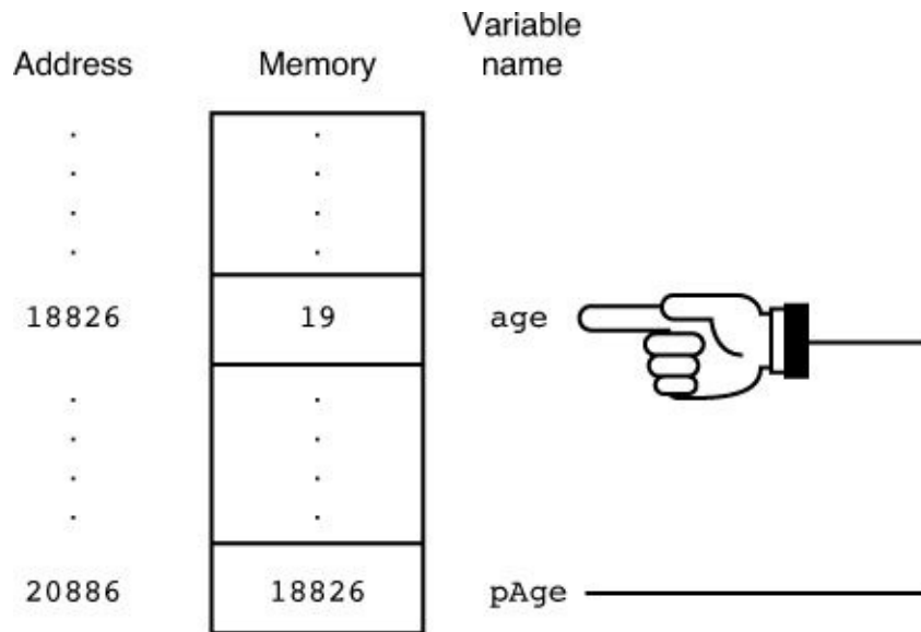
FIGURE 24.1 The variable pAge points to age if pAge holds the address of age .
