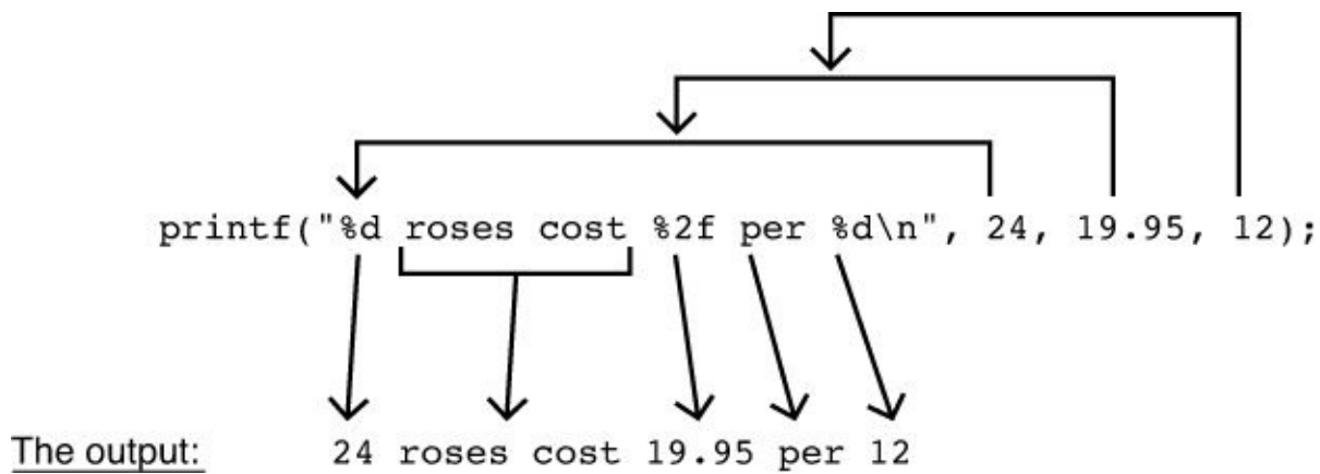
FIGURE 4.1 printf() conversion characters determine how and where numbers print.
