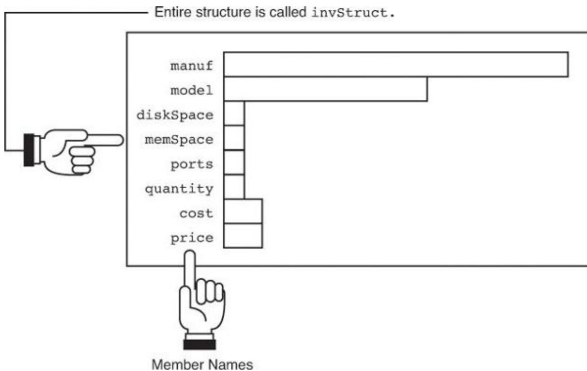
FIGURE 27.1 The format of the invStruct structure.
